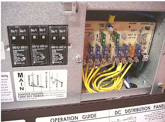
12V House Fuses -Typical View
