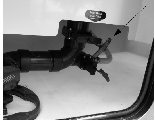
Black Waste Tank Drain Valve (Rear) (Located in water service center) -Typical View
