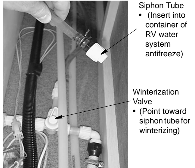
RV Antifreeze Siphon Tube and Winterization Valve (See Drain Valve Location chart at end of this section) -Typical View
