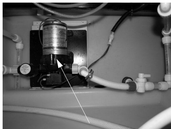
Water Pump -Typical Installation
