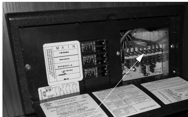
12-Volt House Fuses -Typical View
