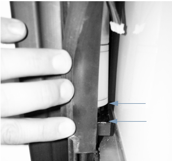
Slideout Motor (Located behind slideout wipe seal) • Use a screwdriver to push slideout motor UP (disengage).
