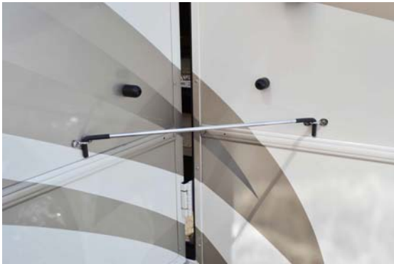
Prop Rod Storage Location (Located on inside of screen door) -Typical View
