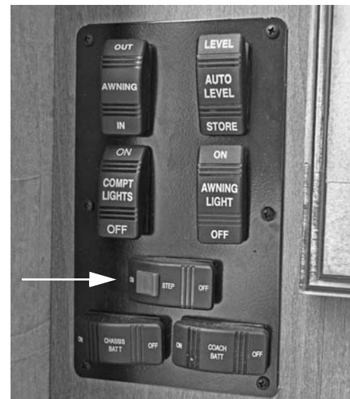
Entry Step Switch (Located near the entrance door) -Typical View
