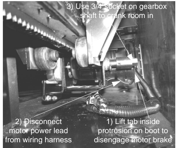
Slideout Motor/Gear Assembly (Located beneath end of slideout room rail) * Shown with slideout room extended -Typical View
