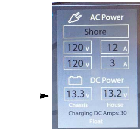
Power Information Screen (Located on “Home” Screen)
