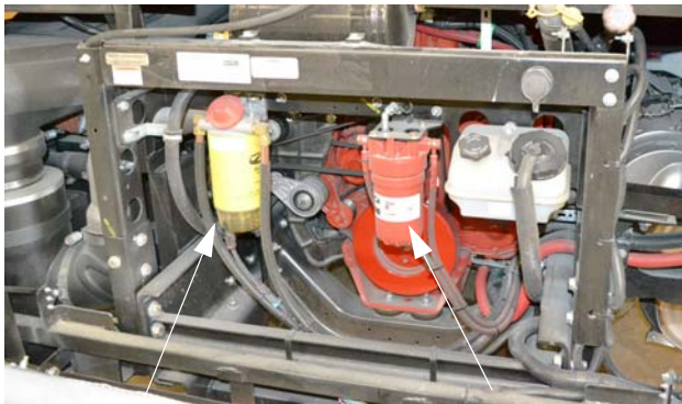
Diesel Fuel/Water Separator (Filter)
