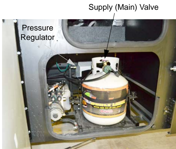
-Typical View
