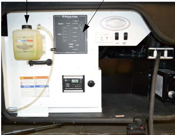
Hydronic Heating System (Located in driver side compartment) -Typical View
