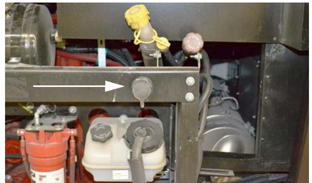
Diagnostic Plug (Located on rear engine compartment shroud) -Typical View
