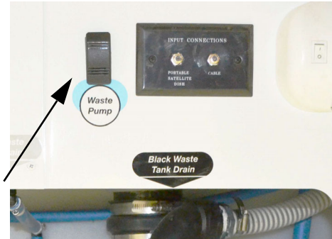
Waste Pump (Located in water service center on driver side of motorhome)
