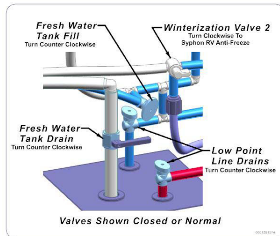
(Located in water service center)
