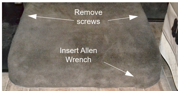
Motor Cover Allen Wrench (Located in the InfoCase)
