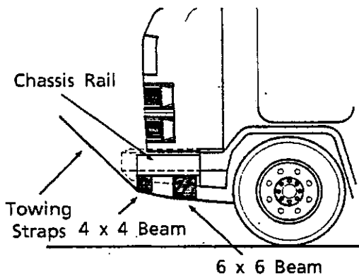
TOWING ATTACHMENT
