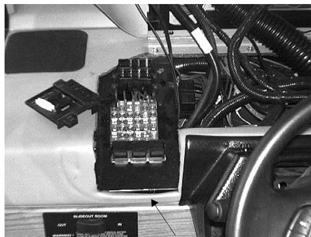
Automotive 12-Volt Fuse Block beneath lift-up dash pod
