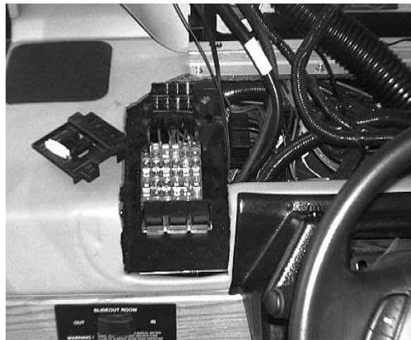
Automotive 12-Volt Fuse Panel Beneath Lift-Up Dash Pod
