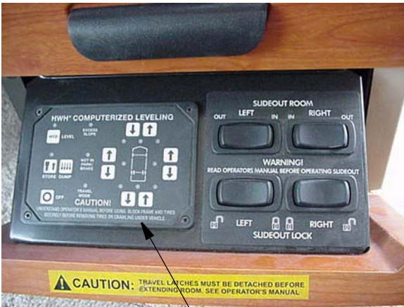
Leveling System Control Panel
