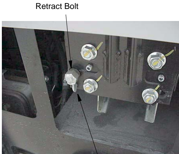
Stop Bolt
