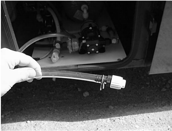
RV Antifreeze Draw Tube in water center or near water pump (insert into container of RV water system antifreeze)
