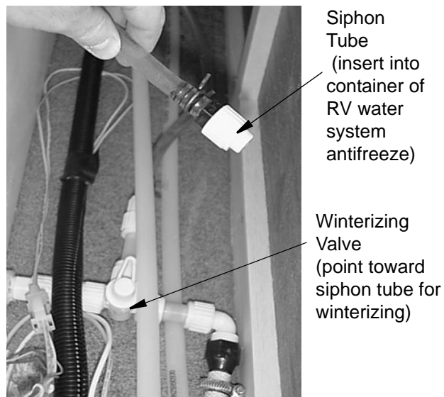
Winterization Valve
