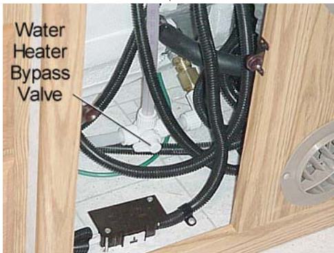
typical installation
