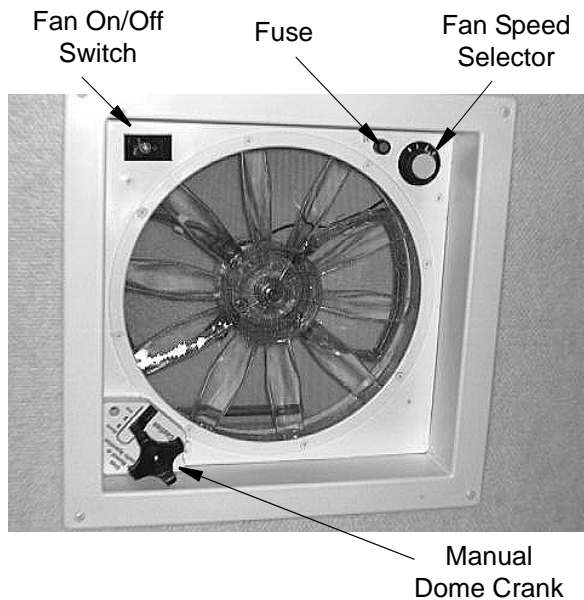
Power Ventilator
