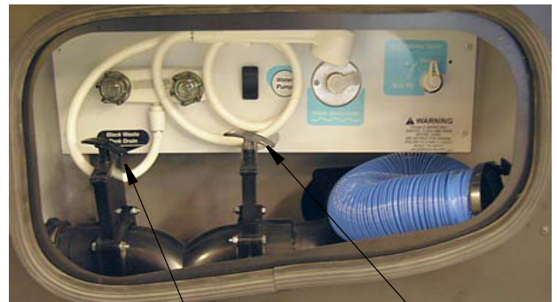
1st - Pull Black handle to drain Black Water (sewage) tank – then close.
