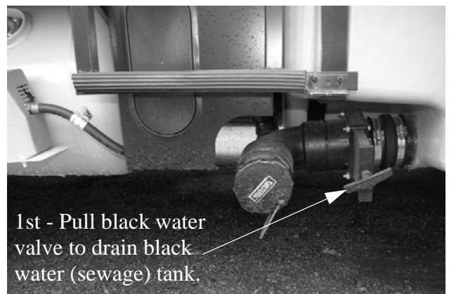
Black Water Drain Valve (Located in driver side compartment) -Typical View
