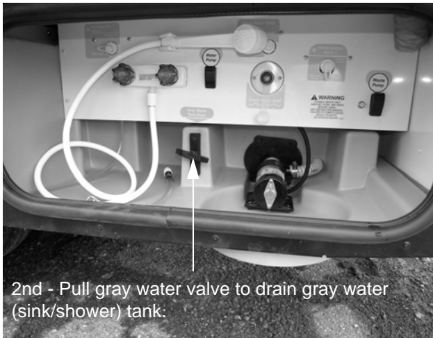
Gray Water Drain Valve (Located inside water service center) -Typical View
