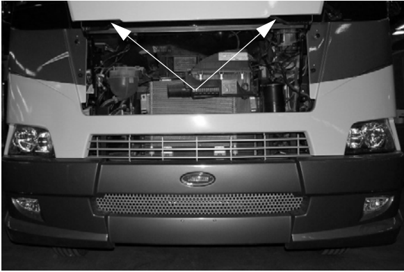
Latch Handle Locations -Typical View
