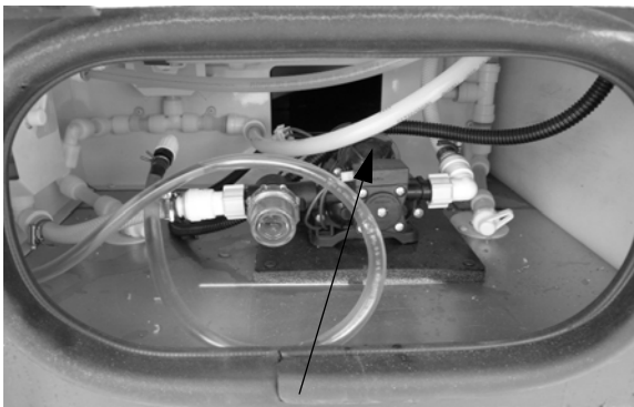
Water Pump (Located in passenger compartment) -Typical Installation
