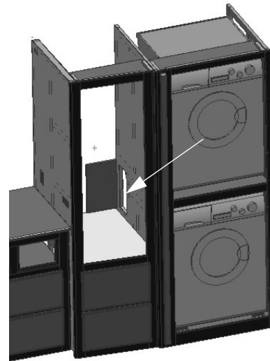
Water Supply Faucets (Located in washer/dryer cabinet behind access door) -Typical View
