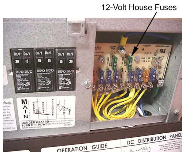
12V Fuse Panel (Located on the right-hand side of the power converter) -Typical View
