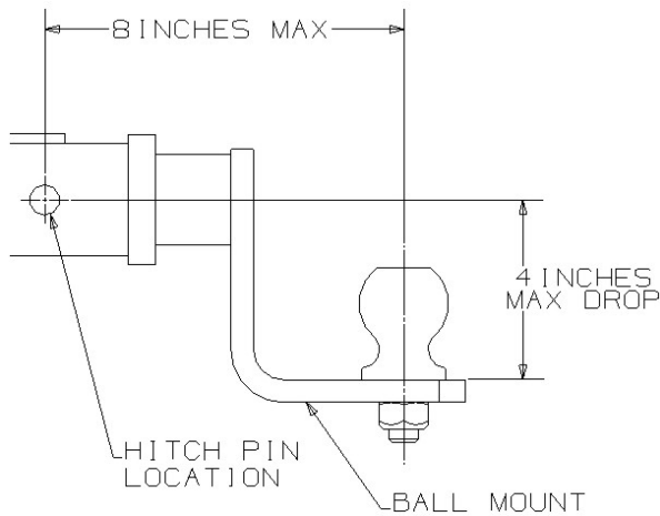
Hitch Assembly
