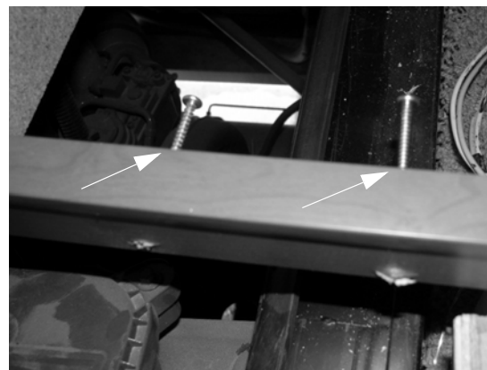
Remove two screws attaching bed board frame to step cover -Typical installation shown
