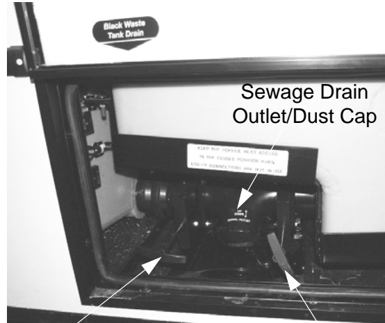
Black Waste Tank Drain Valve Gray Waste Tank Drain Valve
