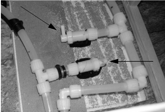
Waterline Drain Valves -Typical installation shown
