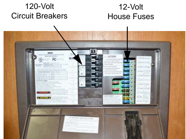
Power Center (Models 27N and 30T) -Typical View
