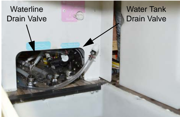
Waterline and Water Tank Drain Valve
