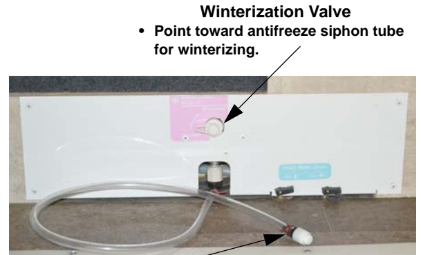
Antifreeze Siphon Tube • Insert into container of RV water system antifreeze.
