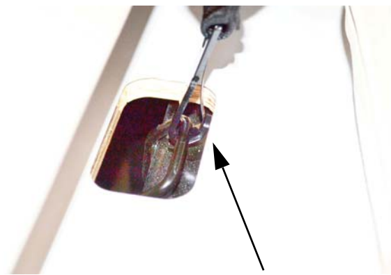
Tether hooked to anchor loop
