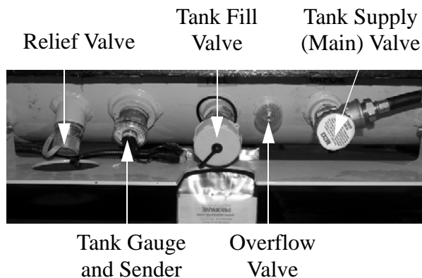
Propane Tank Features -Typical View
