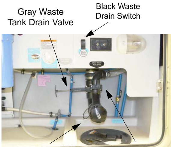
Sewage Drain Outlet/Dust Cap Black Waste Tank Drain Valve
