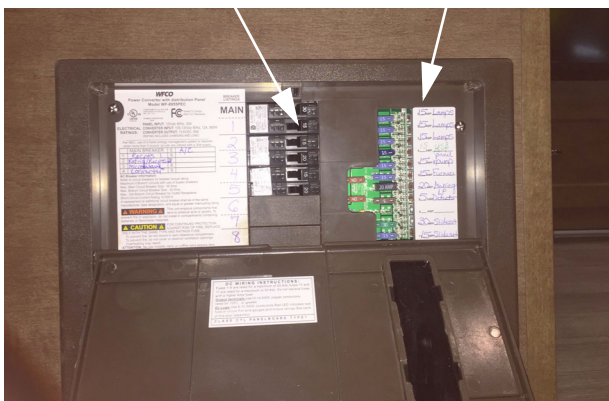
Power Center (Converter) -Typical View
