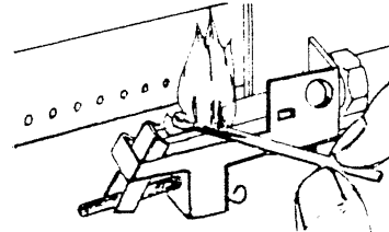
Lighting oven pilot (when pilot is located on the right side of burner.)
