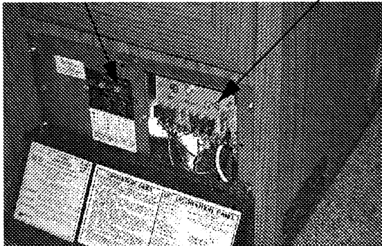
110-Volt Circuit Breaker 12-Volt Coach Fuses
