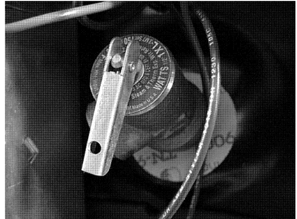
Lift straight out to open P-T valve
