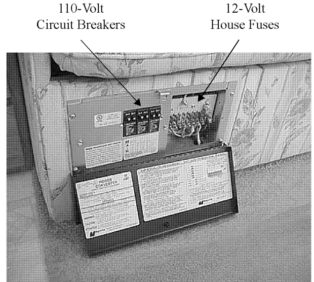
Power Converter
