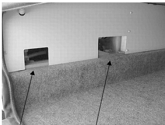
Water Line and Water Tank Drain Valve Access in RH Storage Compartment
