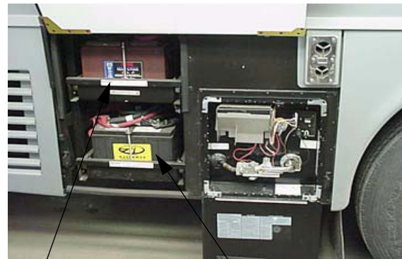
House Batteries
